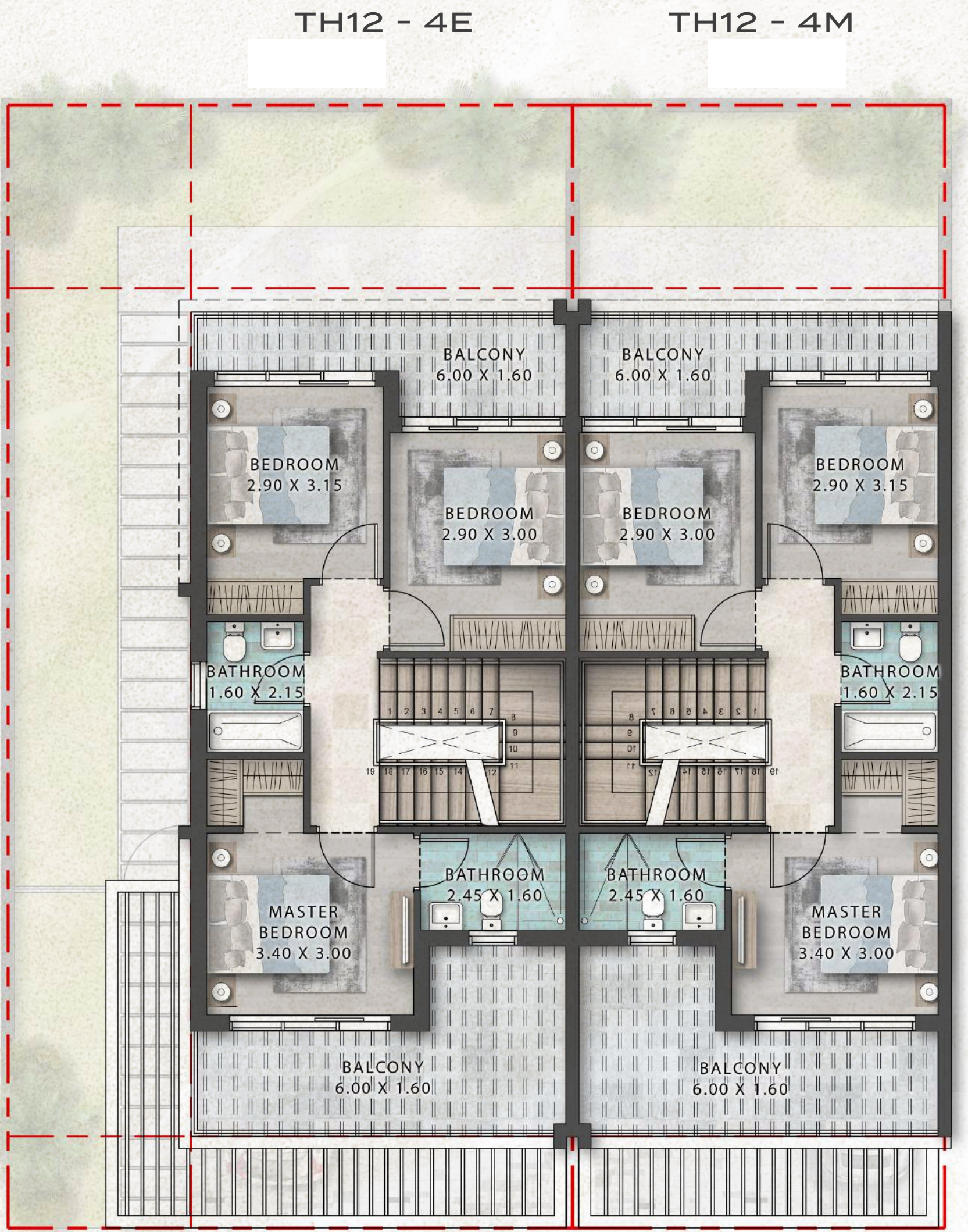
FIRST FLOOR
