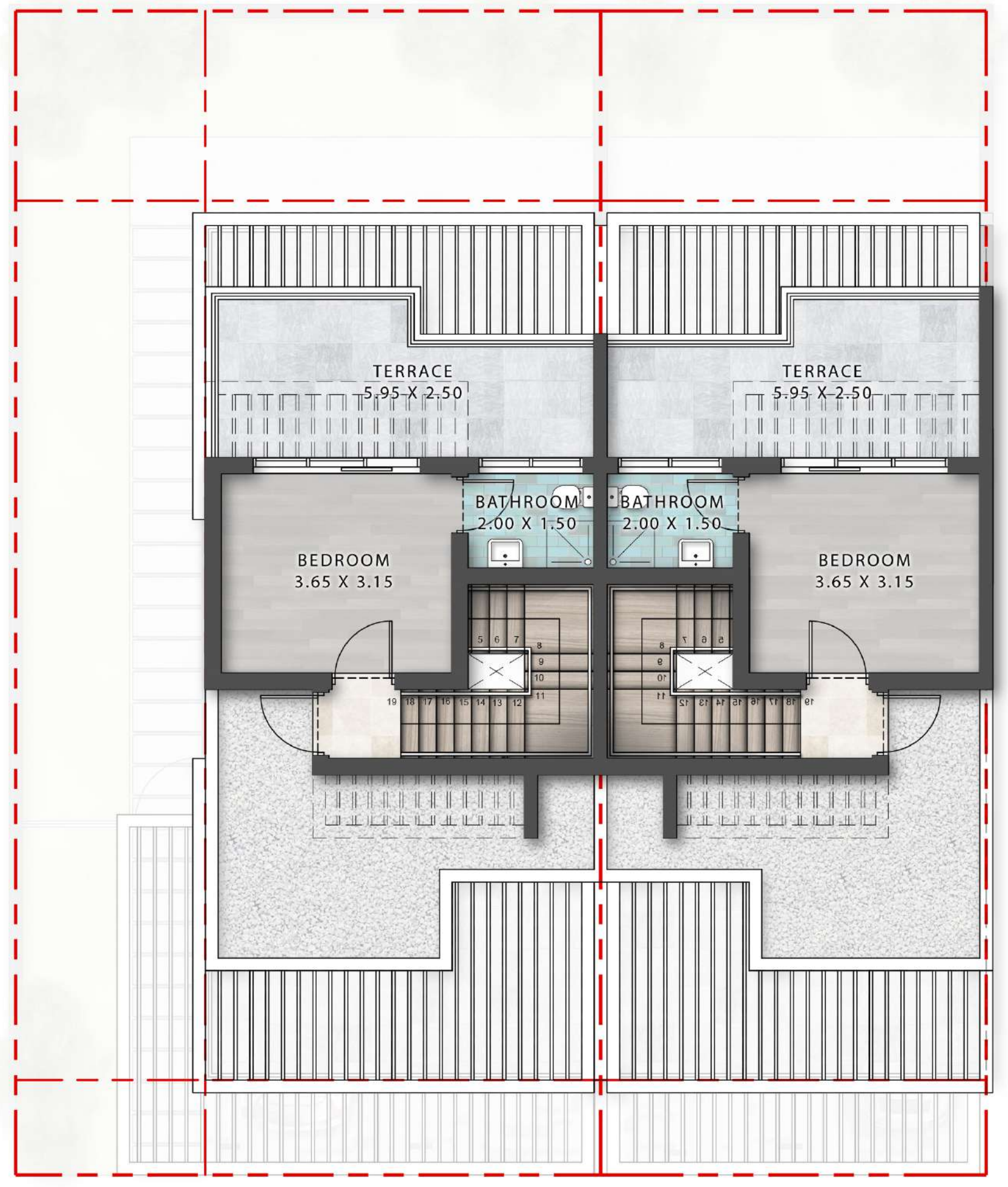
ROOF FLOOR
